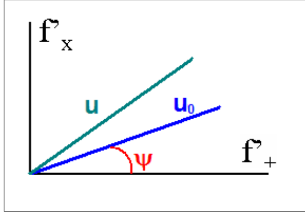
Figure 3.6: Position of the u_0 vector of a regulator and of the associated u vector given from the minimization of the energy disbalance, \psi is the angle between the vector and the f'_+ axis.
