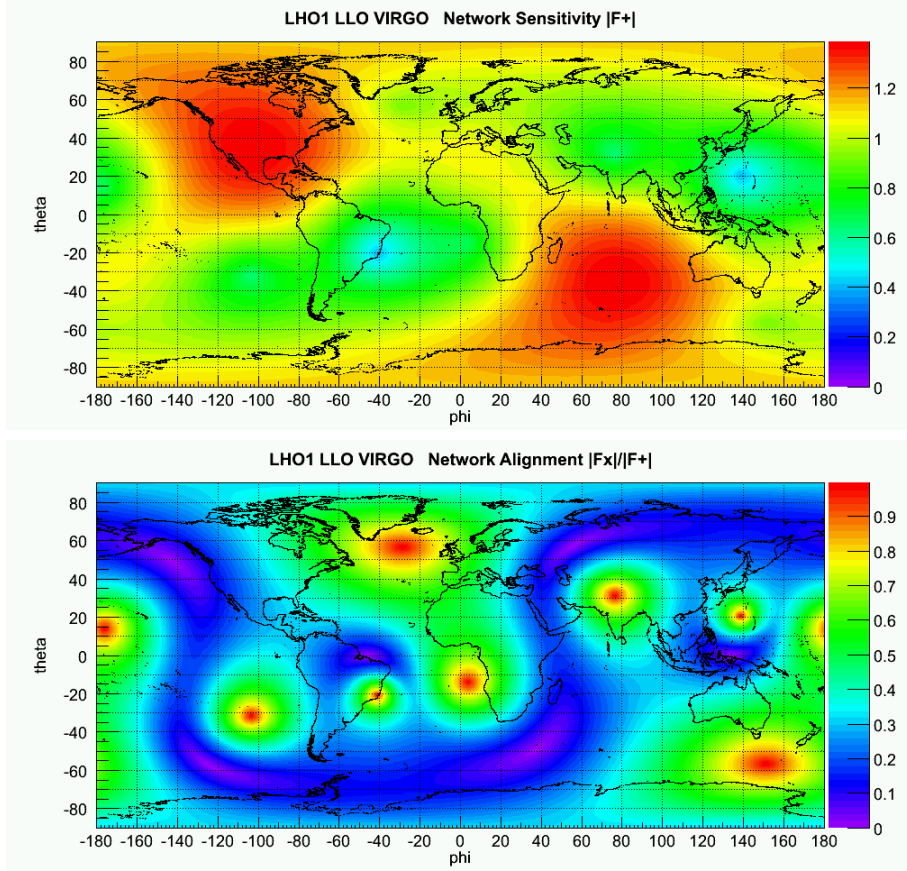
Figure 3.3: Variation of L1H1V1 network antenna patterns in the DPF following earth coordinate: |f'_+| on the top and |f'_\times|/|f'_+| on the bottom. On x -axis is reported the longitude, and on y -axis the latitude. Coloured axis reports valued of antenna patterns.
