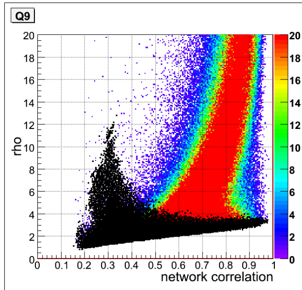
Figure 3.11: Distribution of \rho and cc quantities for background events (black) and simulations (coloured dots). Network is composed of the detectors: L1, H1, H2, V1.
