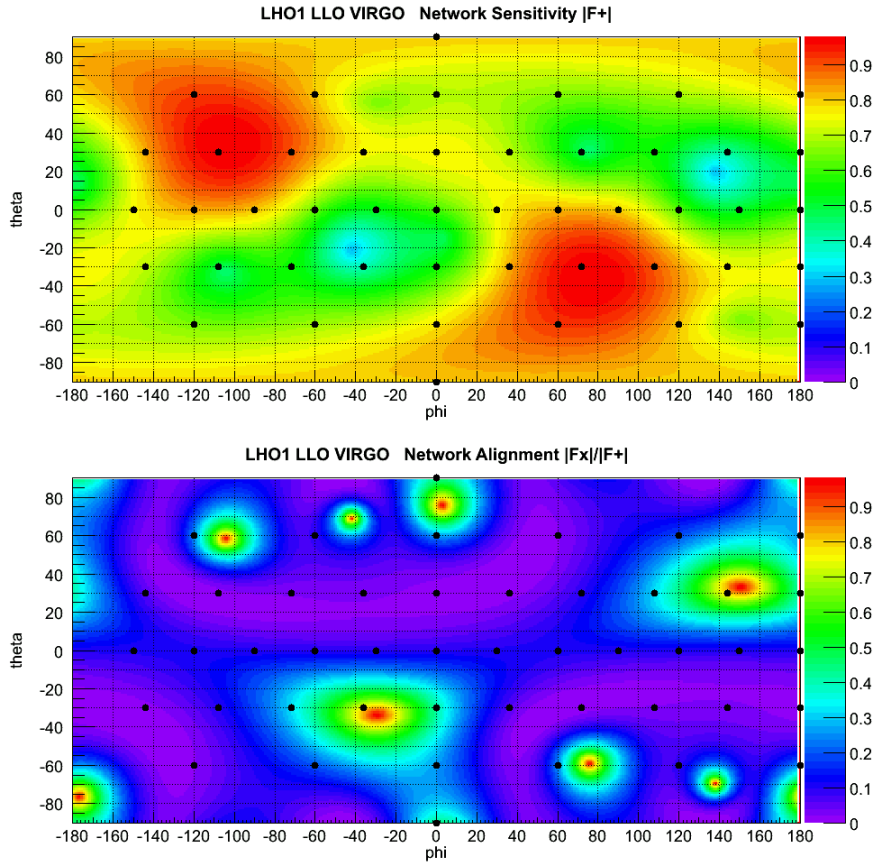
Figure 4.5: The 46 sky positions chosen for the tests of PRC. Coloured background is |f_+| (top) and |f_\times|/|f_+| (bottom) values over the sky, where f_{+,\times} are network antenna pattern defined in the Dominant Polarization Frame.
