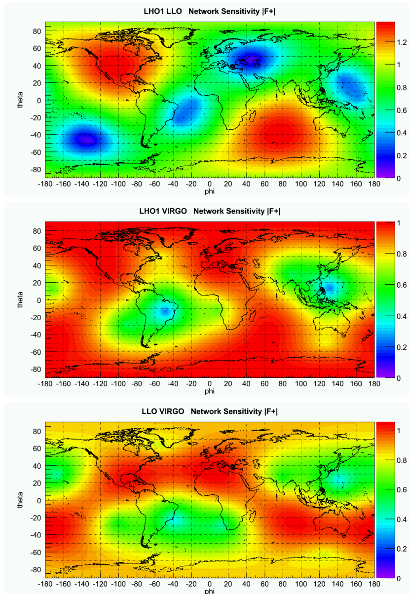
Figure 3.2: Variation of plus component of antenna patterns following earth coordinate for a network of two detectors. On x -axis is reported the longitude, and on y -axis the latitude. Coloured axis reports valued of antenna patterns. From top to bottom the networks are: H1L1, H1V1, L1V1.
