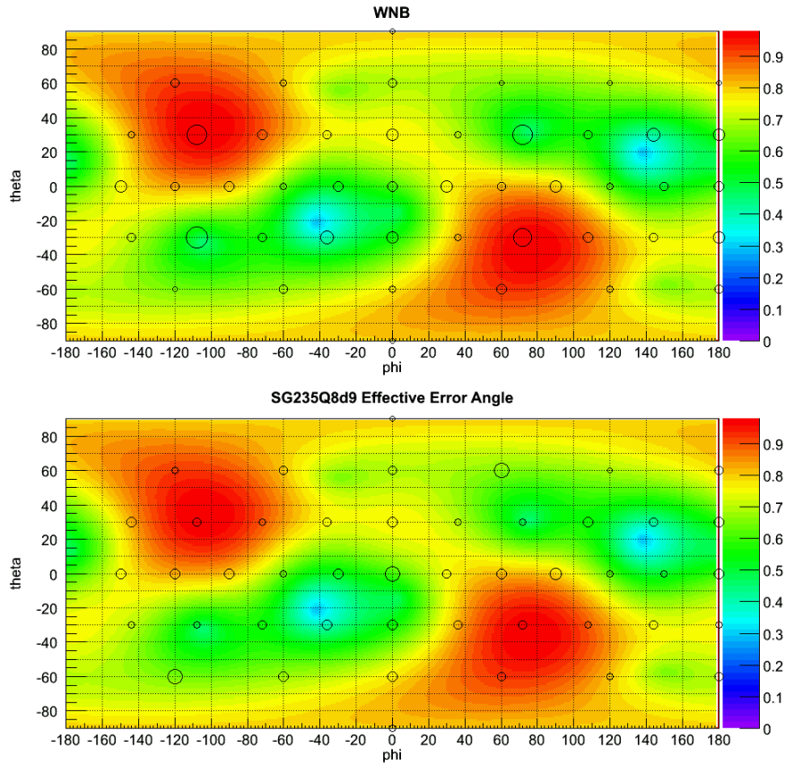
Figure 4.11: Median Effective Error Angle for the 46 tested sky positions for WNB (top) and SGQ9 (bottom) LF waveforms: Bmild search is used for WNB, and Iweak search for SG.
