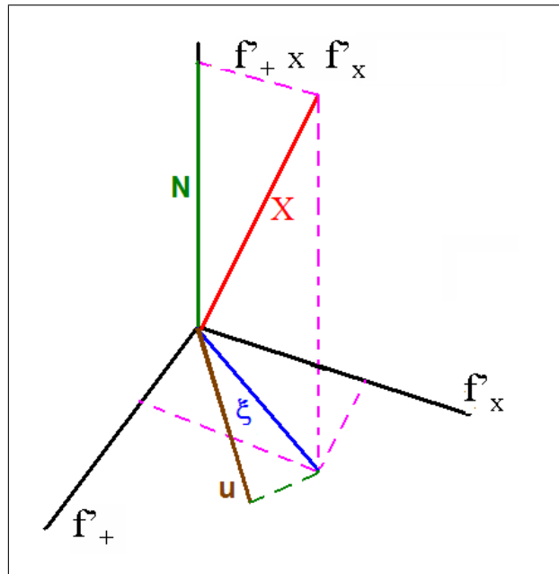
Figure 3.4: Detector response affected by noise (blue) and solution not affected by noise (brown) in the Dominant Polarization Frame
