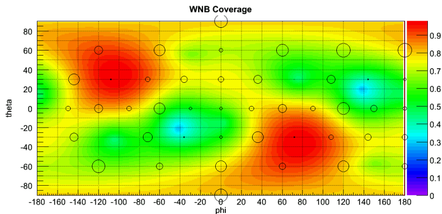
Figure 4.17: Error Region coverage for the 46 tested sky positions and WNB LF waveform, B_{\text{mild}} constrain.
