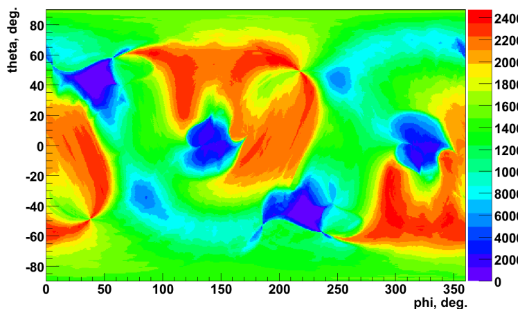
Figure 3.9: Example of the likelihood behaviour as a function of sky coordinates for an event reconstructed from a background analysis.
