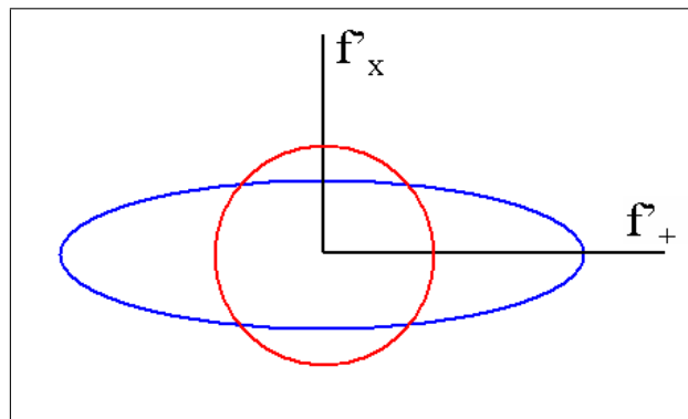
Figure 3.5: Visualization of a circularly polarized signal (red) and of the related detector response (blue) in the Dominant Polarization Frame. Plus component is greater because of the definition of DPF.
